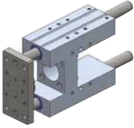
RULMANLI H YATAKLAMALAR (MİL FİYATA DAHİLDİR) (SİLİNDİR HARİÇ) €/Adet
