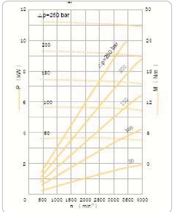
2MF8 Karakteristik Tablosu / Charactenstic Curves Of 2MF8
