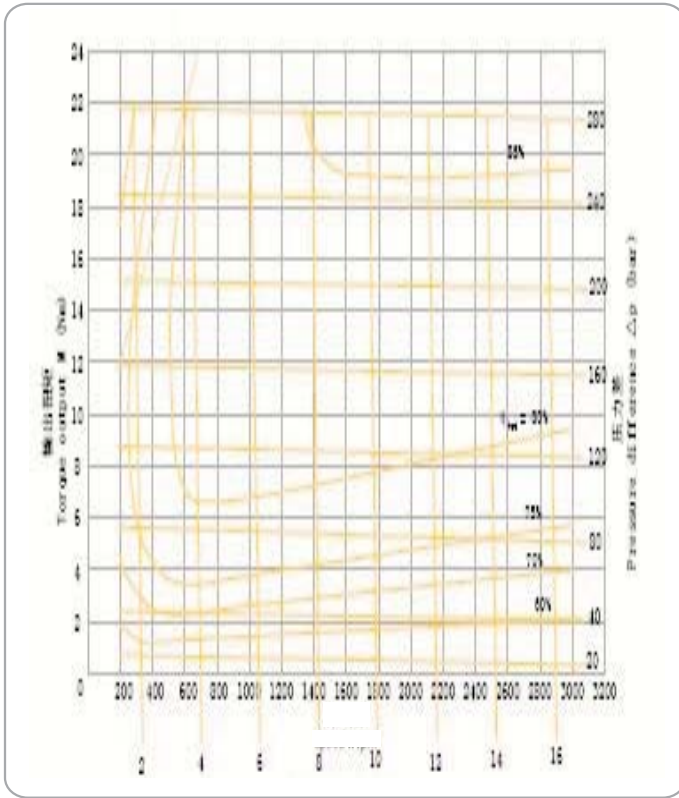
2MF8 Karakteristik Tablosu / Charactenstic Curves Of 2MF8
