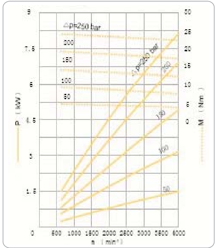
2MF8 Karakteristik Tablosu / Charactenstic Curves Of 2MF8
