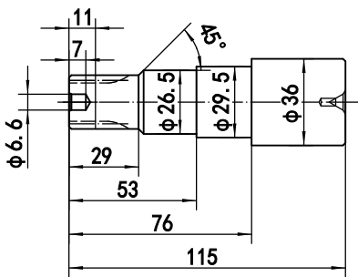
B型标准输入齿轮轴 INPUT GEAR SHAFT (STANDARD TYPE B)
