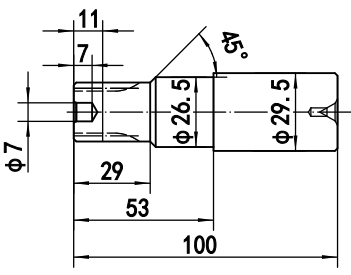
A型标准输入齿轮轴 INPUT GEAR SHAFT (STANDARD TYPE A)
